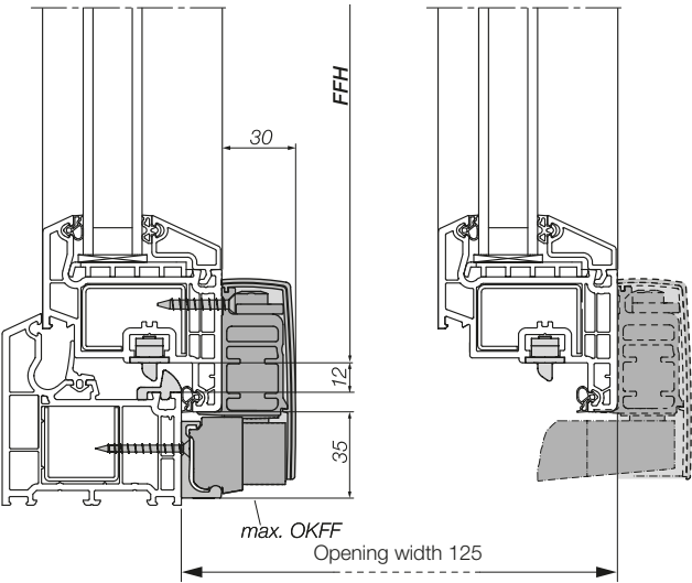
Vertical section ATRIUM HKS® 100 S PVC
