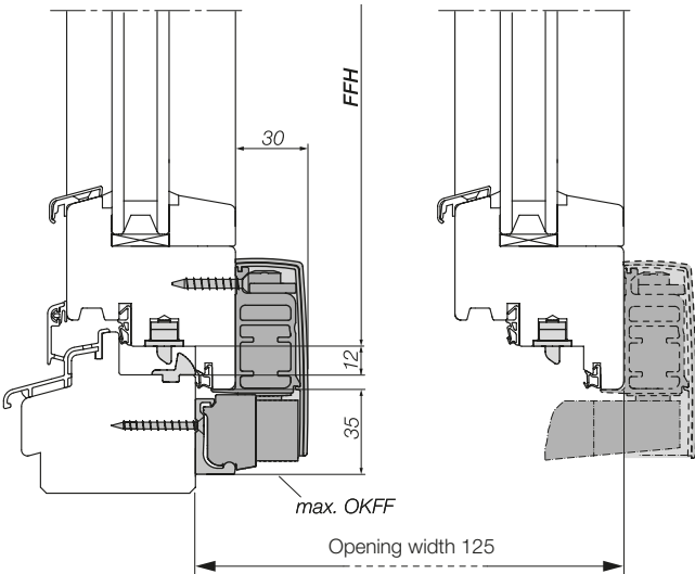
Vertical section ATRIUM HKS® 100 S timber
