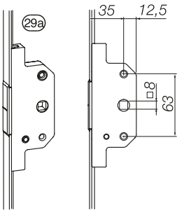
EG French door, b/s 35
