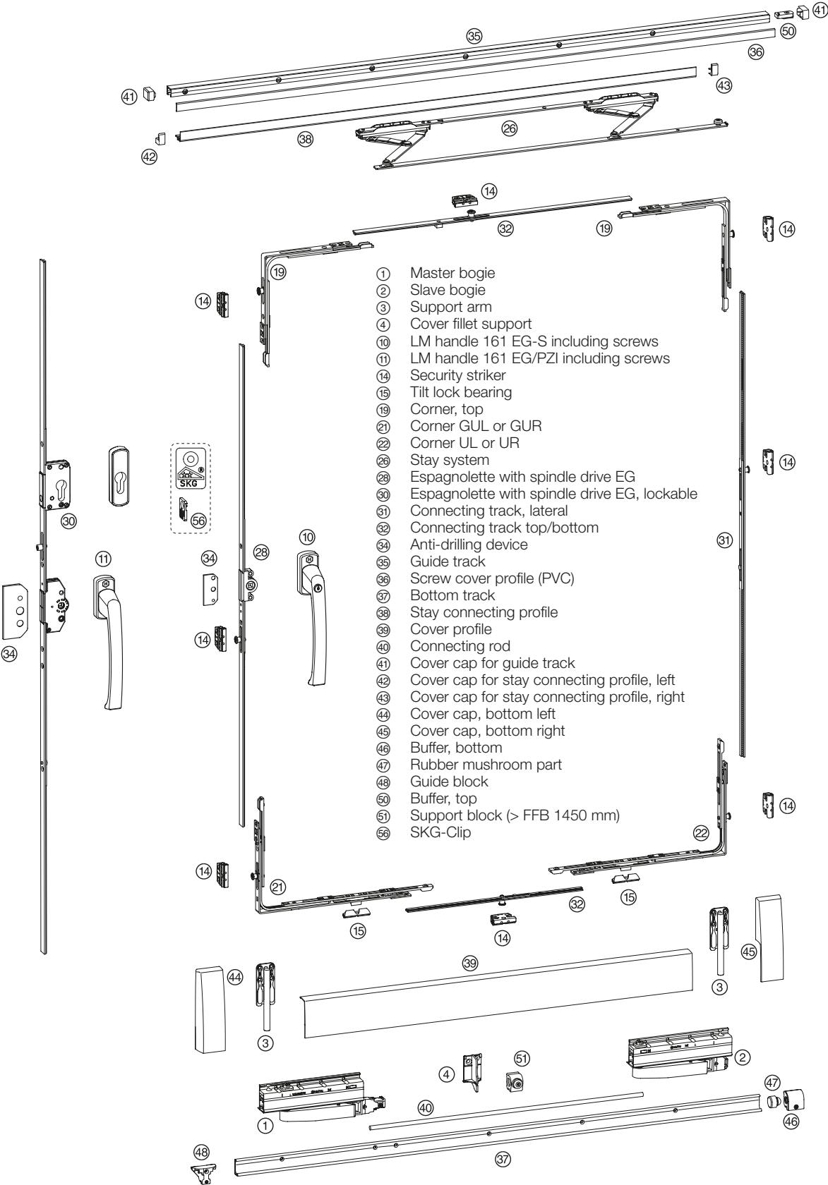
Figure fitting parts = design left (according to DIN EN 12519 opening to the right)
