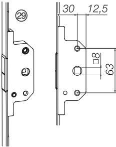
EG French door, b/s 30
