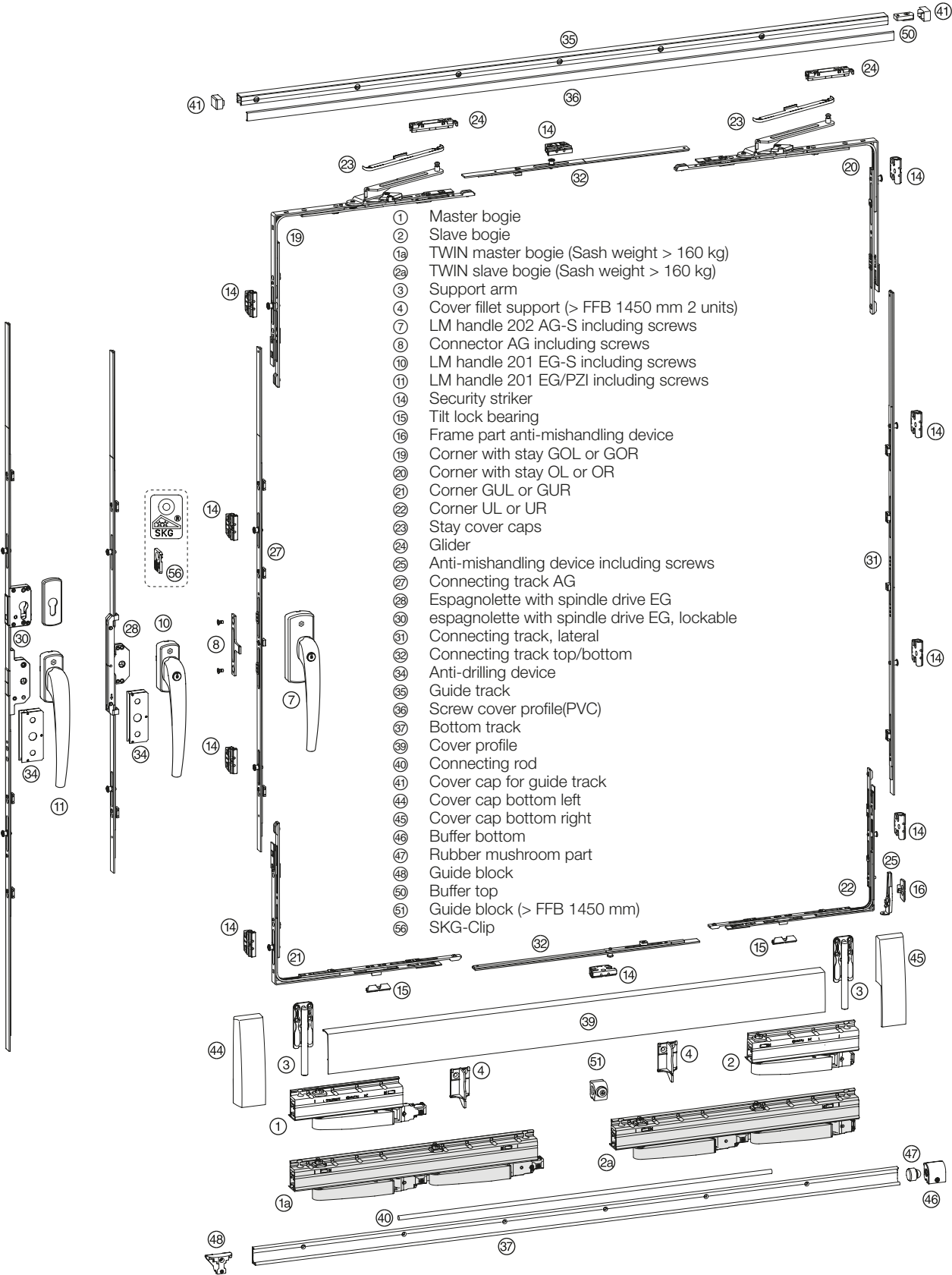
Figure fitting parts = design left (according to DIN EN 12519 opening to the right)
