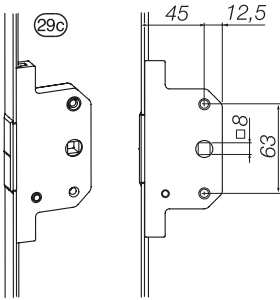
EG French door, b/s 45
