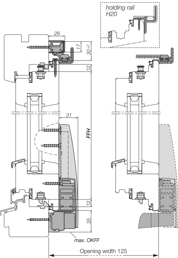
Vertical section ATRIUM HKS® 160 S timber
