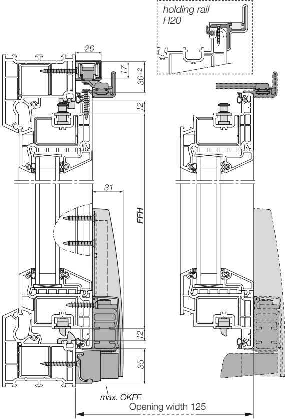
Vertical section ATRIUM HKS® 160 S PVC
