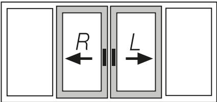
Scheme C Four-part element: 2 sliding sashes (L and R) with mounting posts between HKS elements
