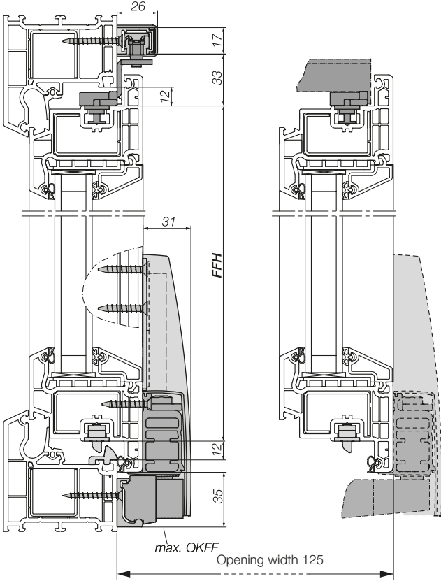
Vertical section PVC
