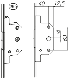
EG French door, b/s 40
