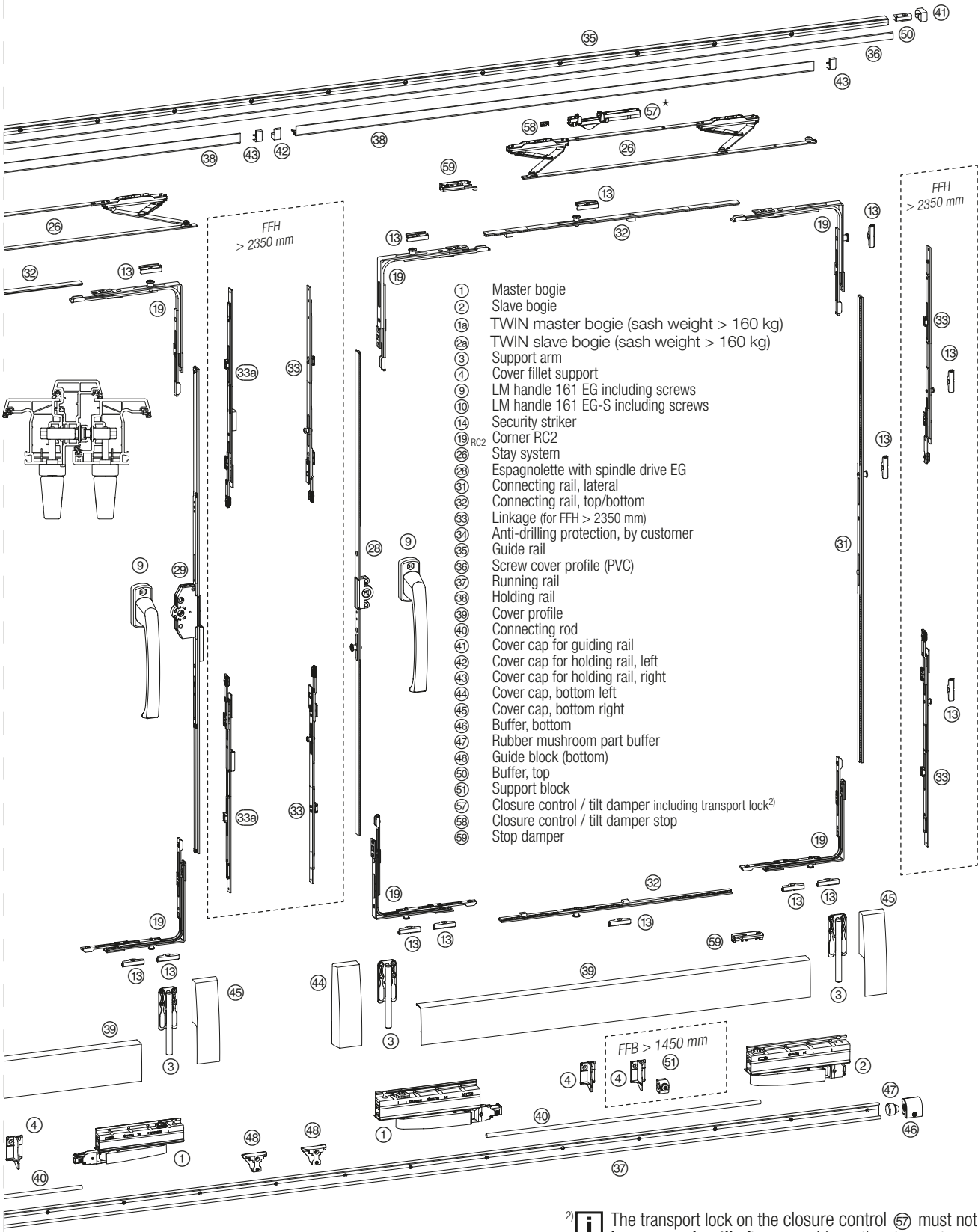
Figure fitting parts = design left (opening to the right according to DIN EN 12519)
