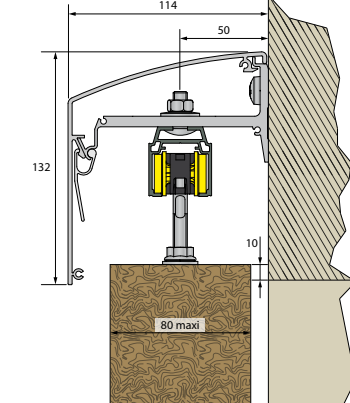
Fixation murale (brise-soleil)
